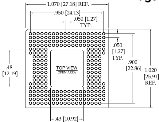
Fig. 21 255 Pins Thru-Hole: 10-20-06-255-400T4-R27-L14 Surface Mount: 10-20-06-255-414T4-R27-L14 Rollerball®: 10-20-06-255-RB501T4-R27-L14
