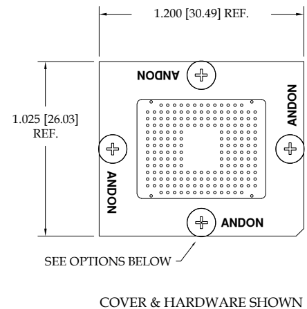
Fig. 12 230 Pins Thru-Hole: 694-230D-TH-491-R27-L14-1 Surface Mount: 694-230D-SM-500-R27-L14-1 Rollerball®: 694-230D-SM-RB593-R27-L14-1
