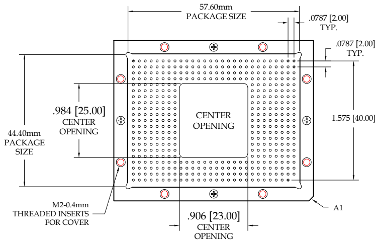
Fig. 19 431 Pins Thru-Hole: 692-431-TH-491-R27-L14 Surface Mount: 692-431-SM-500-R27-L14 Rollerball®: 692-431-SM-RB593-R27-L14
