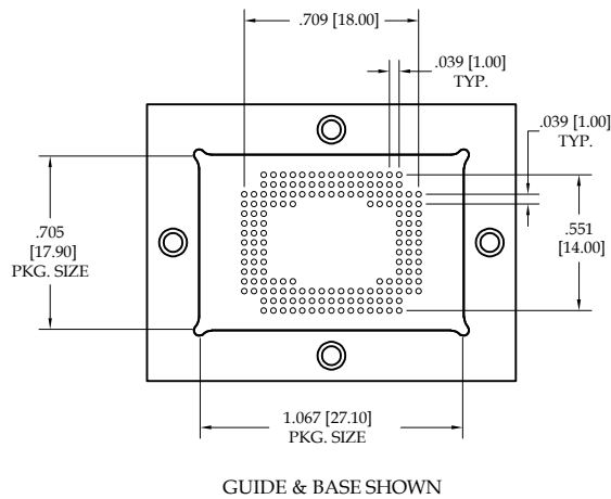
Fig. 11 163 Pins Thru-Hole: 694-163B-TH-491-R27-L14-1 Surface Mount: 694-163B-SM-500-R27-L14-1 Rollerball®: 694-163B-SM-RB593-R27-L14-1
