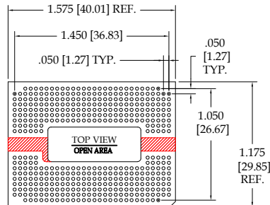
Fig. 16 454 Pins Thru-Hole: 10-30-15-454- 274UM -R27-L14 Surface Mount: 10-30-15-454- 315UM -R27-L14 Rollerball®: 10-30-15-454- RB338UM -R27-L14 REFER TO LAST PAGE FOR CARRIER OPTIONS RED SECTIONS OF INSULATOR CAN BE OMITTED AND THIS CARRIER USED IN THEIR PLACE: Carrier/Sips: 9-10-30-15A-454-XXX-R27-L14-SIP
