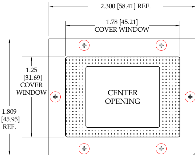
Fig. 19 431 Pins Thru-Hole: 692-431-TH-491-R27-L14 Surface Mount: 692-431-SM-500-R27-L14 Rollerball®: 692-431-SM-RB593-R27-L14
