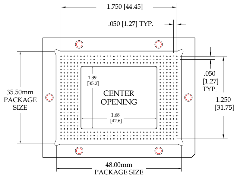
Fig. 20 455 Pins Thru-Hole: 683-455-TH-491-R27-L14-1 Surface Mount: 683-455-SM-500-R27-L14-1 Rollerball®: 683-455-SM-RB593-R27-L14-1
