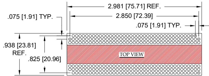
Fig. 22 231 Pins Thru-Hole: 10-39-05-231-400T4-R27-L14 Surface Mount: 10-39-05-231-414T4-R27-L14 Rollerball®: 10-39-05-231-RB501T4-R27-L14 REFER TO LAST PAGE FOR CARRIER OPTIONS RED SECTIONS OF INSULATOR CAN BE OMITTED AND THIS CARRIER USED IN THEIR PLACE. Carrier/Sips: 9-10-39-05-231-XXX-R27-L14-SIP Replace "XXX" with choice of terminal
