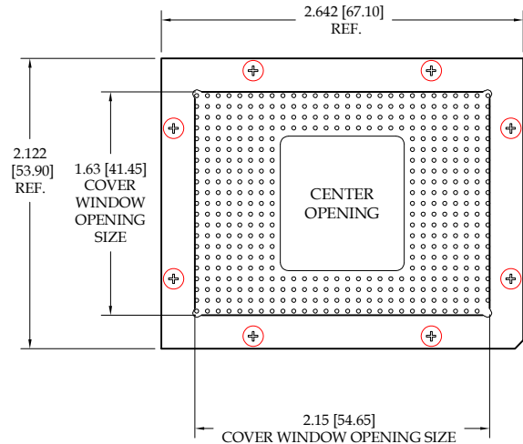
Fig. 19 431 Pins Thru-Hole: 692-431-TH-491-R27-L14 Surface Mount: 692-431-SM-500-R27-L14 Rollerball®: 692-431-SM-RB593-R27-L14
