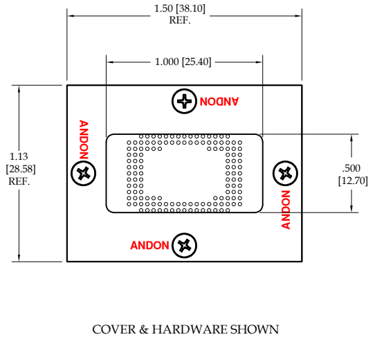
Fig. 11 163 Pins Thru-Hole: 694-163B-TH-491-R27-L14-1 Surface Mount: 694-163B-SM-500-R27-L14-1 Rollerball®: 694-163B-SM-RB593-R27-L14-1
