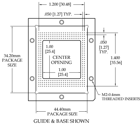
Fig. 26 284 Pins Thru-Hole: 683-284-TH-491-R27-L14 Surface Mount: 683-284-SM-500-R27-L14
