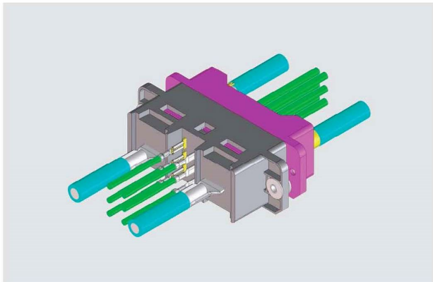
Receptacle side connector
