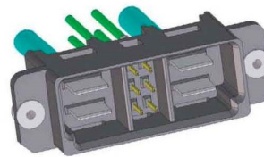
Plug side connector
