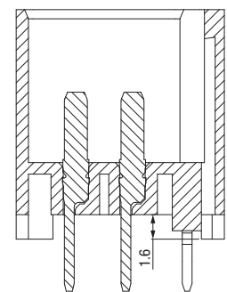
X-X' Cross section (With the contact inserted)
