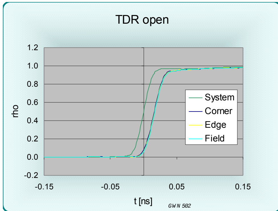
Figure 5 TDR signal from an OPEN circuited 113003-200Y test socket
