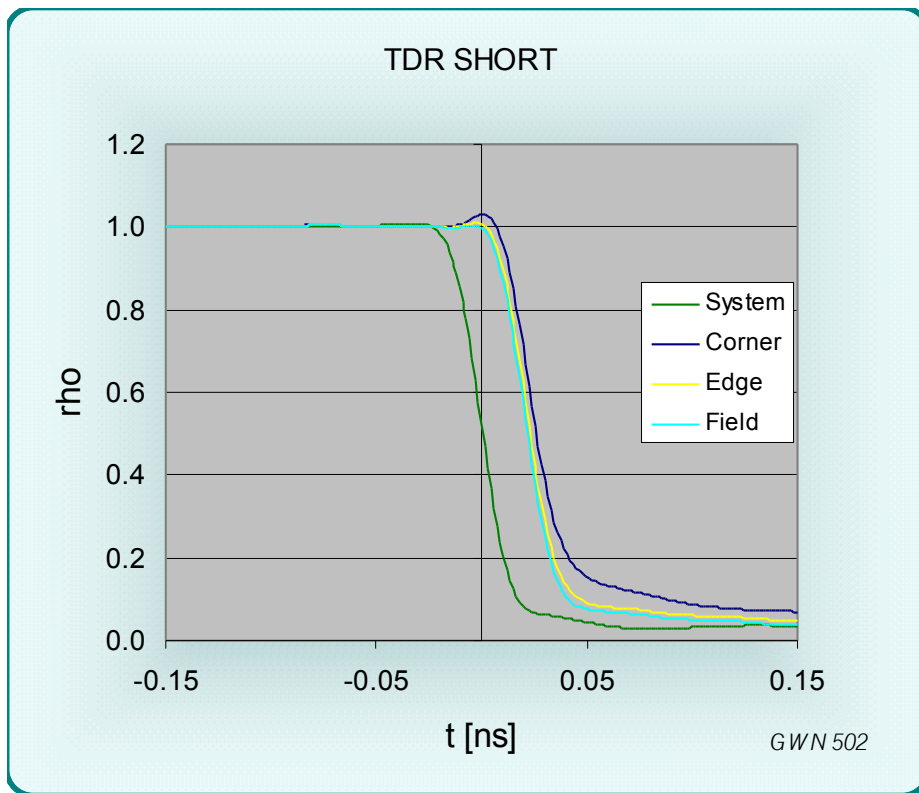
Figure 6 TDR signal from a SHORT circuited 113003-200Y test socket
