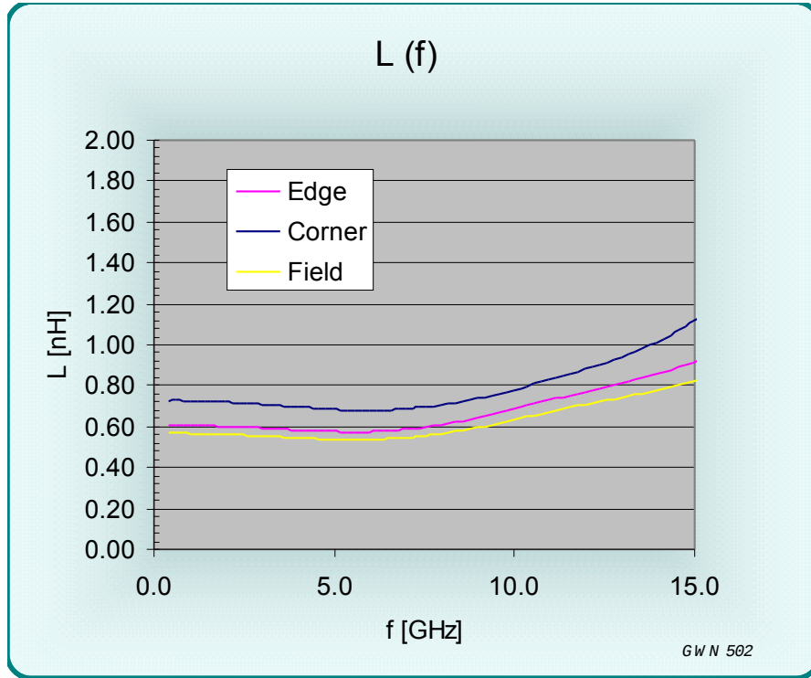
Figure 15 L(f) for the 113003-200Y test socket
