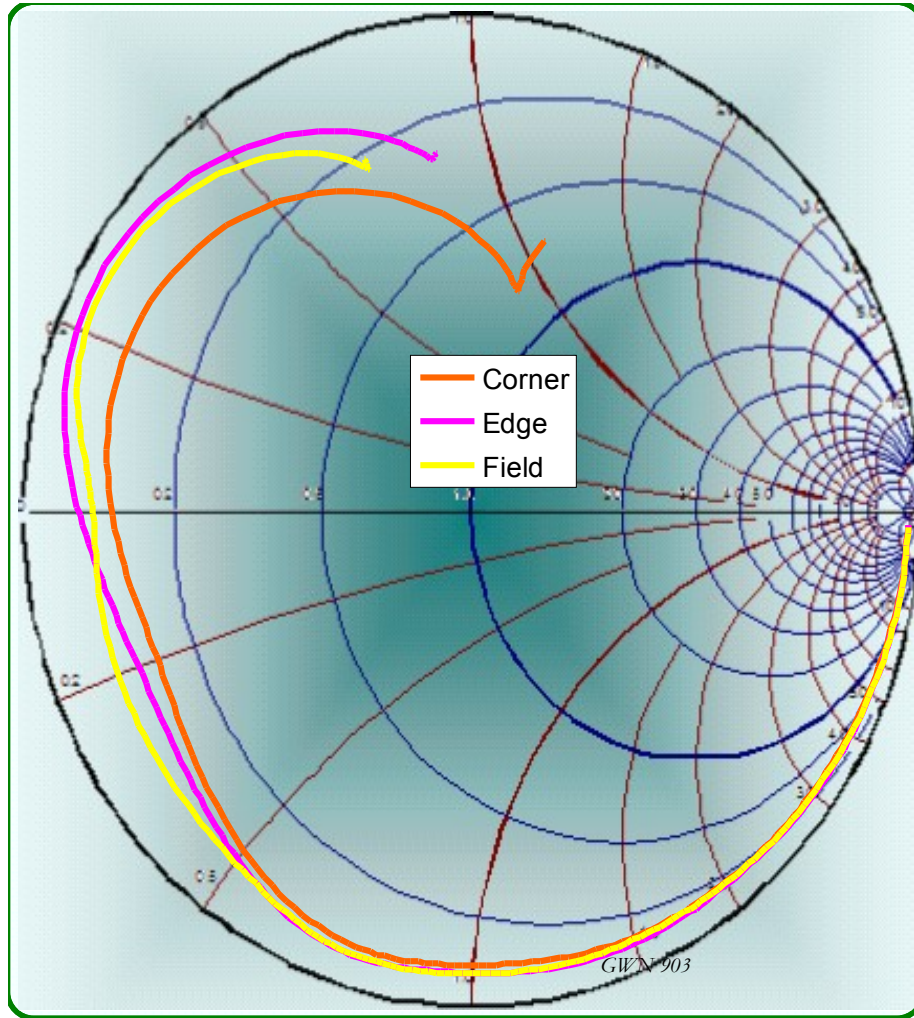
Figure 12 Reflections from the open circuited 113003-200Y test socket
