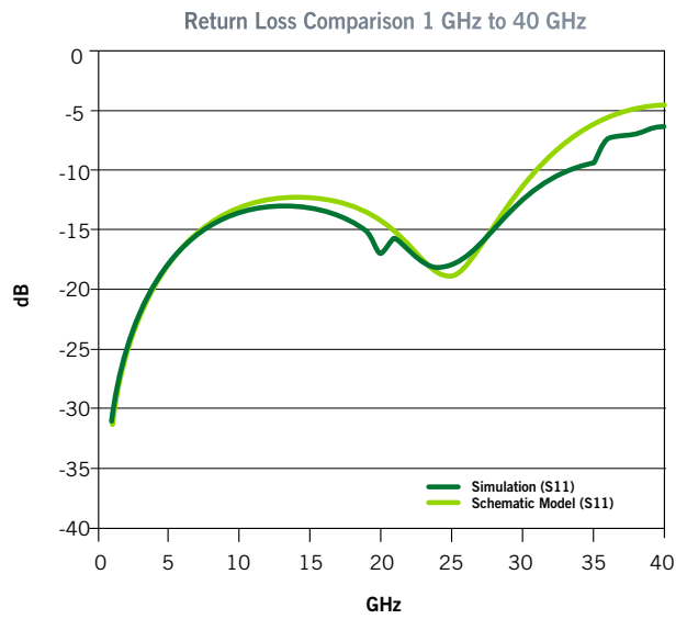
Figure 6. GSG P2A Return Loss, 0.8 mm pitch
