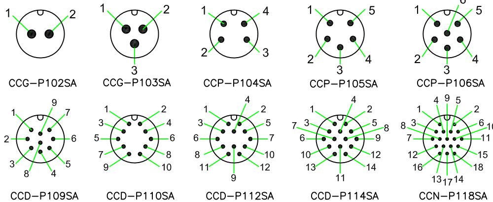
PIN ASSIGNMENT FRONT VIEW (前視圖)
