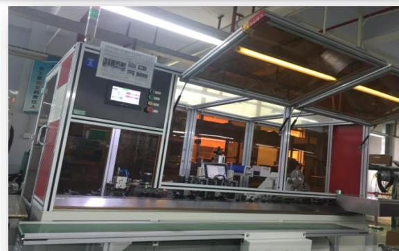
Wire Pre-treatment Machine (Stripping wire skin/trim shielding braid/Stripping AL mylar / copper foil)
