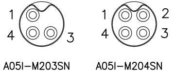
PIN ASSIGNMENT FRONT VIEW (前視圖)
