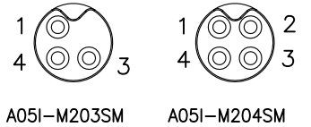
PIN ASSIGNMENT FRONT VIEW (前視圖)
