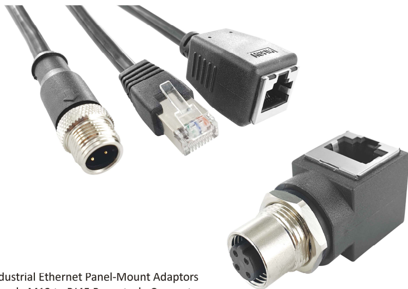
RJ45 to M12 Patch cord , A / D / X Coding
