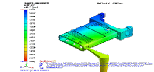
Injection Analysis
