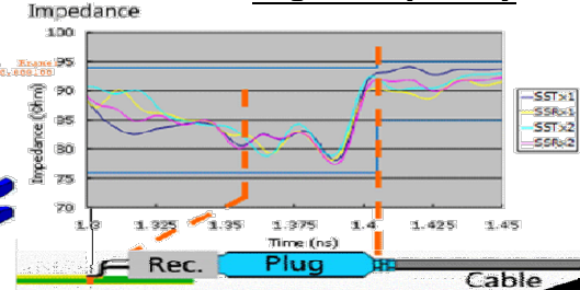
High Frequency
