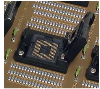
Loranger LGA Socket on Loranger Humidity / HAST Printed Circuit Board
