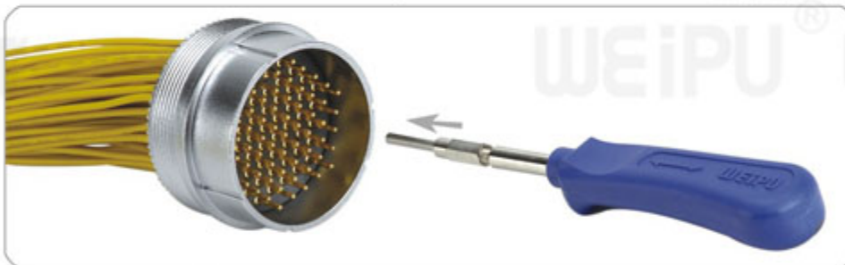
Remove contact
