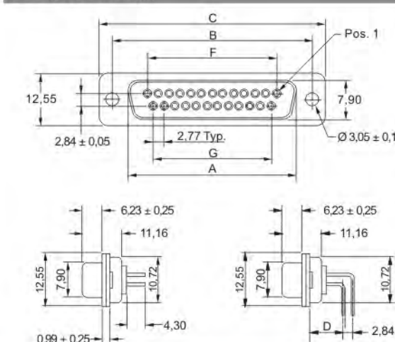
Socket connector
