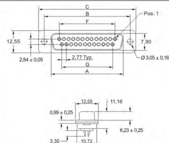
Socket connector
