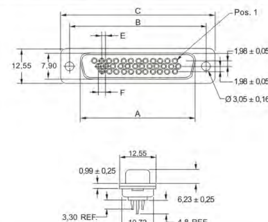
Socket connector
