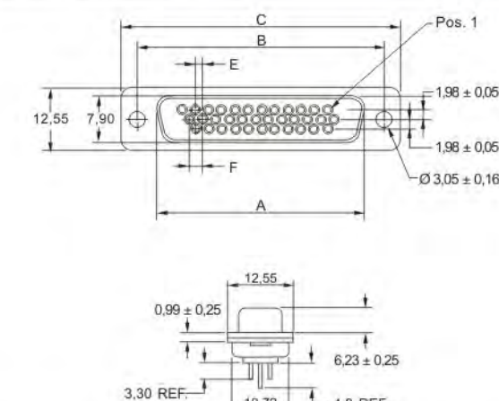
Socket connector
