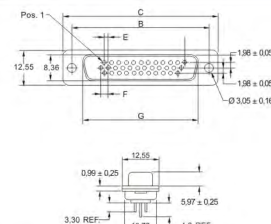
Plug connector
