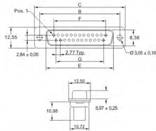
Plug connector
