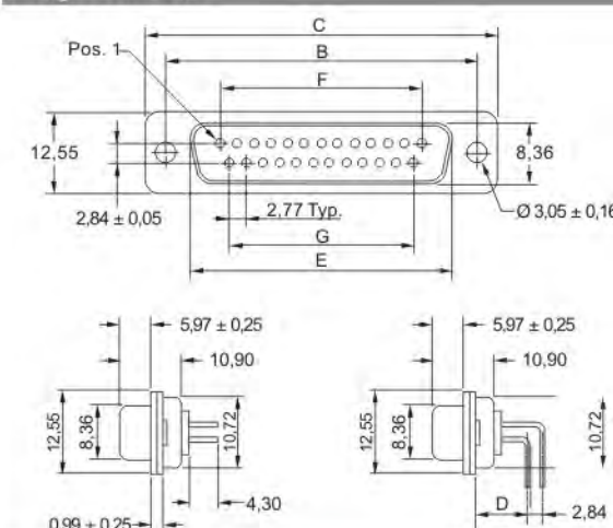
Plug connector
