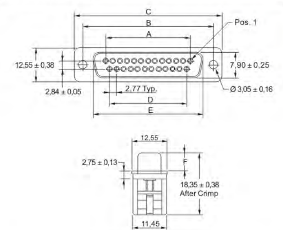
Socket connector
