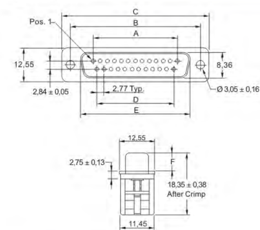
Plug connector
