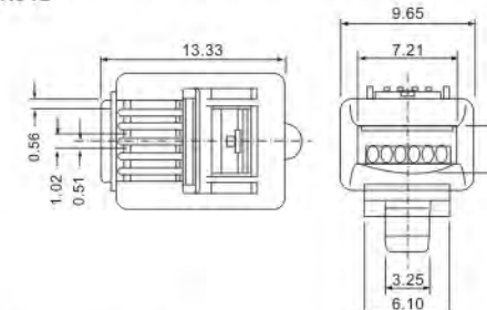
Six Conductor / Six Position Line Cord Plug RJ12
