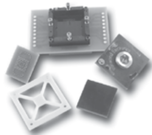
GHz Bandwidth Wire-in Elastomer Socket for Samsung's eMMC SG-BGA-7219 is found on pg 10
