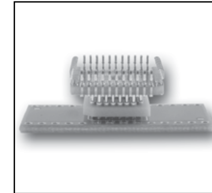
DIP to PLCC Package Converter
