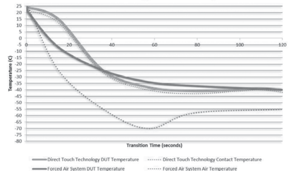
Direct Touch Technology vs. Forced Air System
