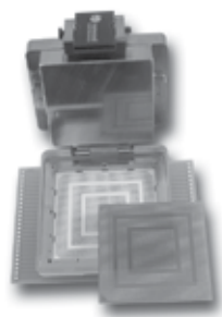
Stamped Spring Pin BGA ATE Socket for LTE Femtocell SoCs CBT-BGA-6015 is found on pg 9
