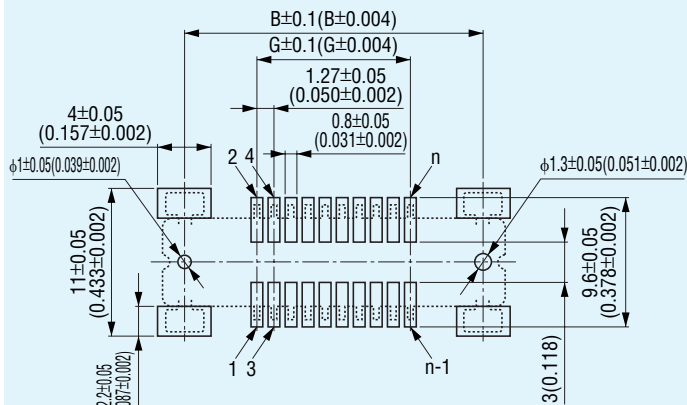
Printed Circuit Board Layout (Component Side View)
