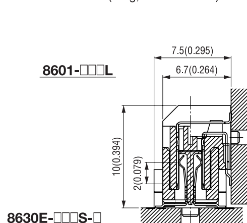
Mating for Board to board connector (8601 series : Vertical mating)
