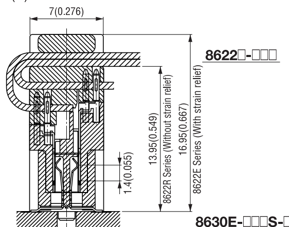
Mating for Board to cable connector (8622E / 8622R series)
