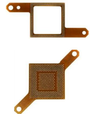
POP Interposers
