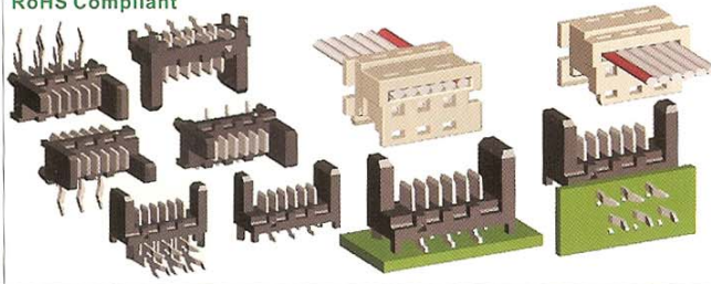
1.27mm IDC Connector Right
