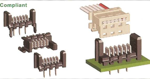
1.27mm IDC Connector Straight Type.
