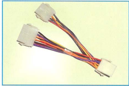
(3x4)M+(8M+12M)
