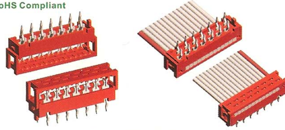
2.54mm IDC Connector (Paddle Board Type).
