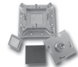
Production test Stamped Spring Pin Socket for QFN with ePad & manual lid CBT-QFN-xxxx is found on pg 9
