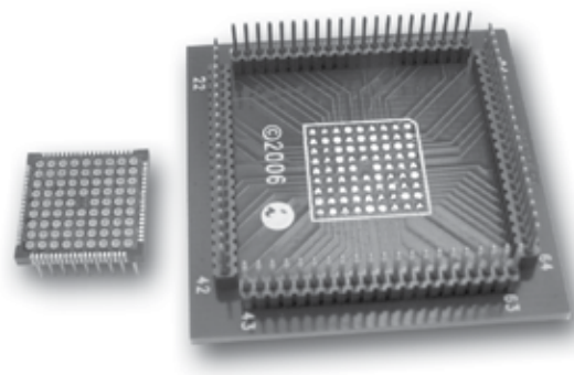
QFP Probing Adapter
