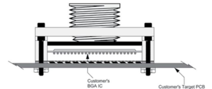
27mm, 20 Watt BGA GHz Socket
