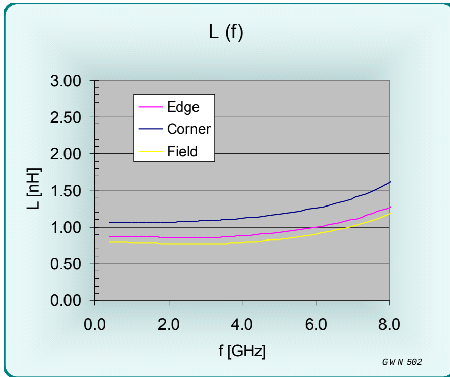
Figure 15 L(f) for the BGA connector
