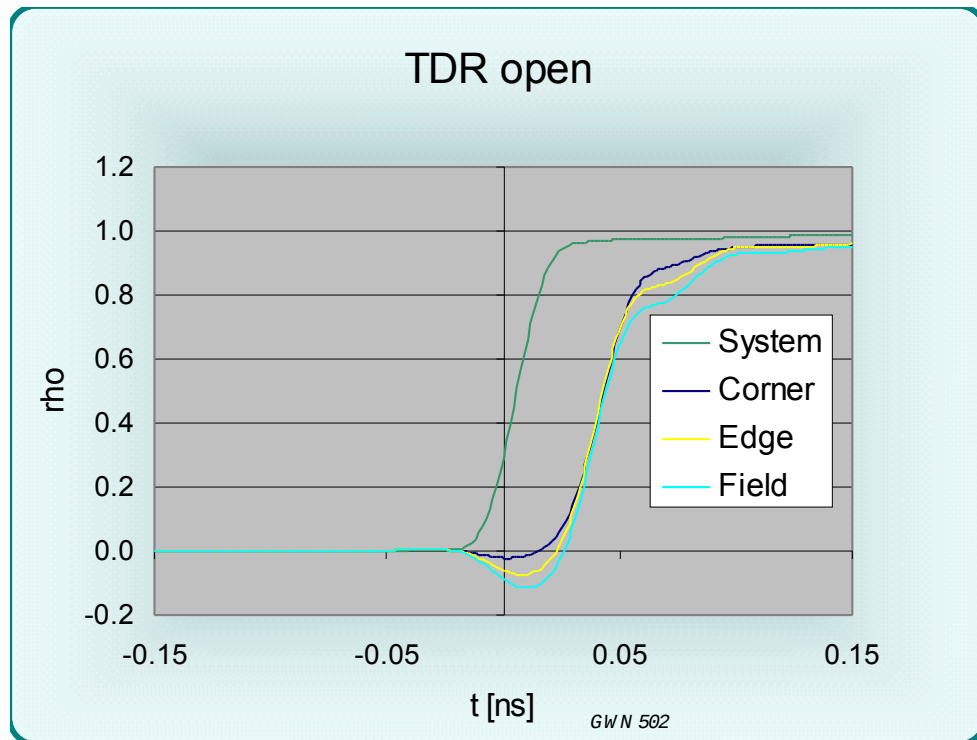
Figure 5 TDR signal from an OPEN circuited BGA connector
