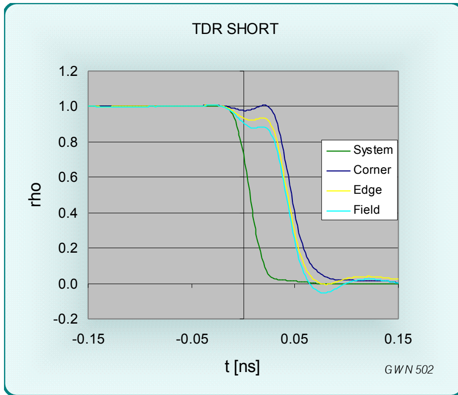
Figure 6 TDR signal from a SHORT circuited BGA connector
