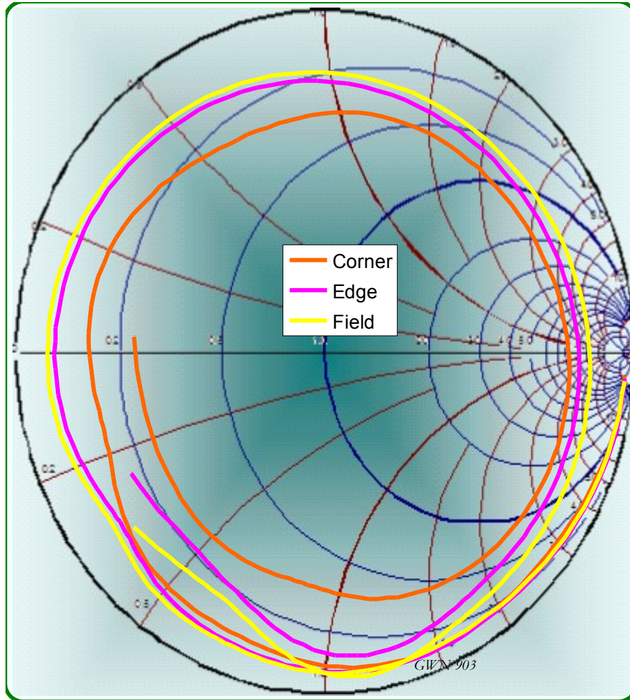
Figure 12 Reflections from the open circuited BGA connector
