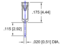
- 75 Terminal Shown
