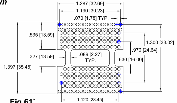
Fig.61* 205 Pins
