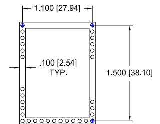
Fig.46 32 Pins Thru-Hole: 575-16-26-032-01S-R29-L14 Surface Mount: 575-16-26-032-93S-R29-L14
