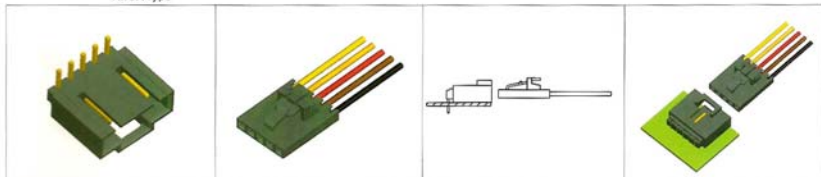
3750S-XX No. Of Positions S: Straight Type R: R/A Type
