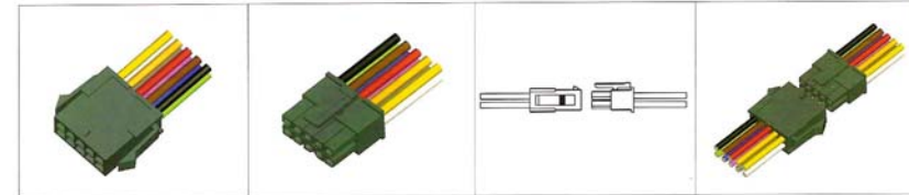
5561-XX No. Of Positions Plug Housing Double Rows
